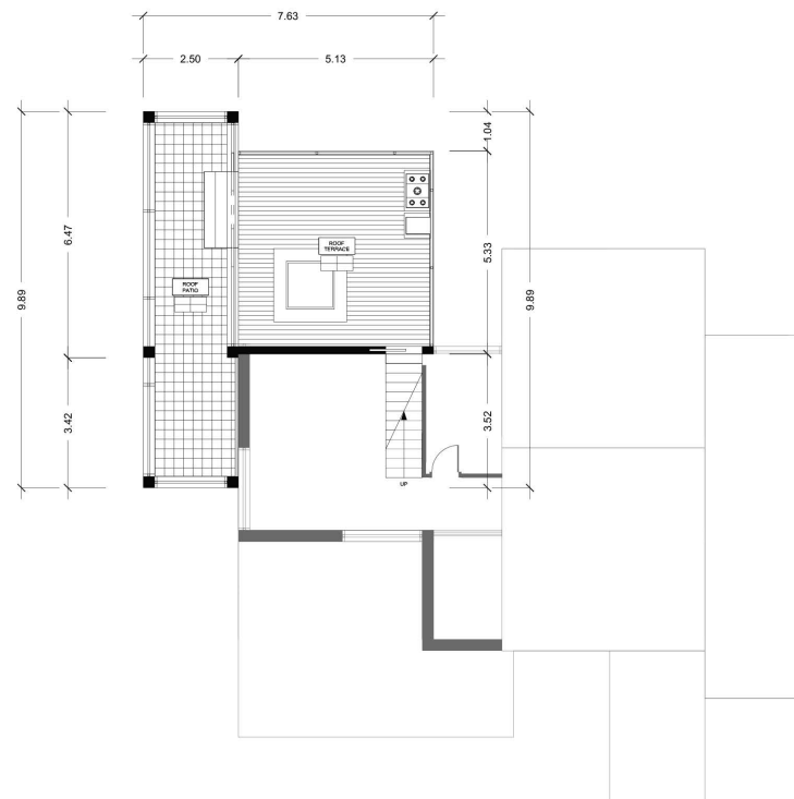
FLOOR 2
