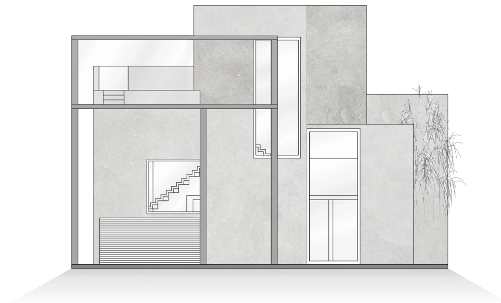
4 WEST ELEVATION 1:200
